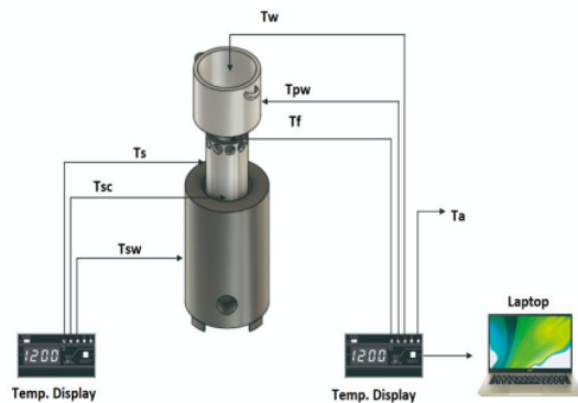
Figure 2. Experimental installation
