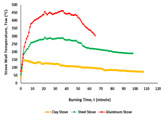
Figure 4. Stove wall temperature history
