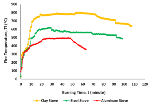
Figure 3. Fire temperature history
