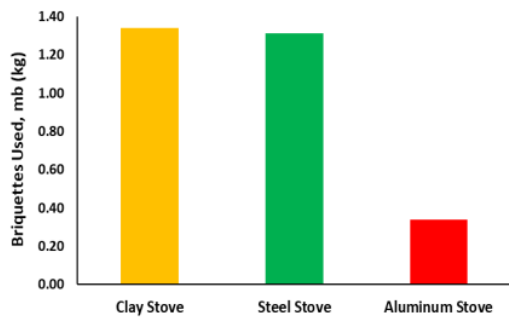
Figure 6. Mass of briquettes used
